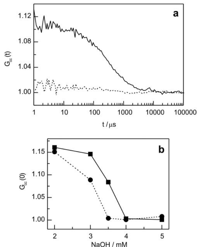
Figure 1. Hybridization detection with single molecules. (a) Cross-correlation curves of two different combinations of library and blocker oligonucleotides. Solid line: library 04 and blocker B0, perfect match. Dashed line: library 05 and blocker B0, mismatch of 4 bp. All oligonucleotide concentrations were 10 nM (in 1\times SSC buffer). An aliquot of 3.5 mM NaOH was added for permissive conditions. Both traces are the average of five individual measurements. (b) Effect of NaOH concentration on the initial amplitude of the cross-correlation curve, G_{cc}(0) . Squares: library 04 and blocker B0, perfect match. Circles: library 05 and blocker B0, mismatch of 4 bp.
