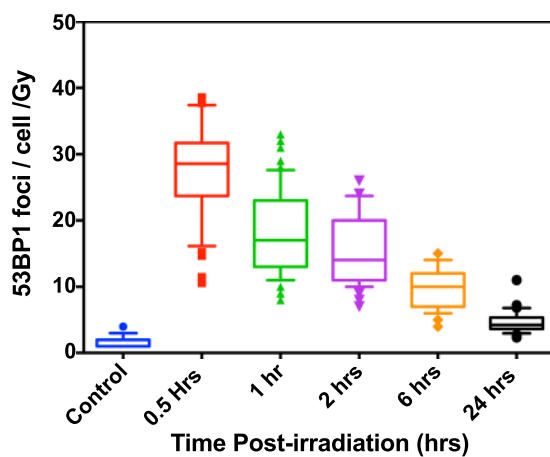
Figure 3. Quantitative analysis of the variations in 53BP1 foci per cell per Gy in AG01522B cells after exposure to 10 MeV (LET-4.6 keV/ \mu m) laser-accelerated protons shown as whisker box plots generated using Prism 6 software. The lower part of the box indicate first quartile, the dividing line shows the median and top line shows the third quartile of the 53BP1 foci per cell per Gy. The lower and upper ends of the whisker indicate 10 th and 90 th percentile also indicating the outliers below 10 th percentile and above 90 th percentile. The number of cells considered for each data point ranged from 50–300 in three independent replicates.
