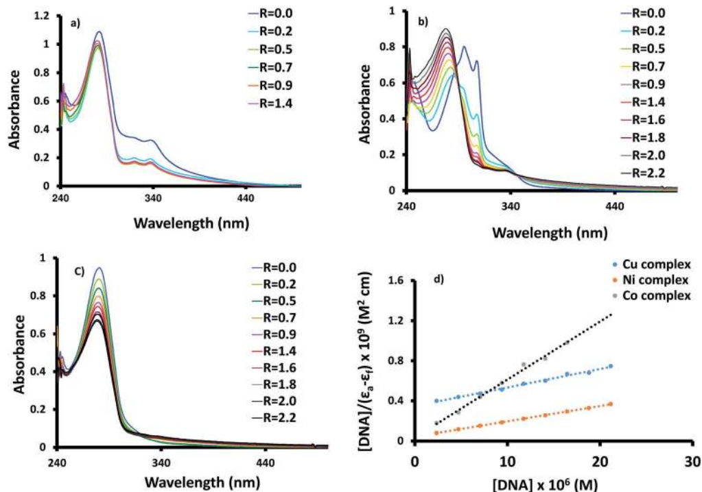
Fig. 3 Absorption spectra of complexes (a) 1, (b) 2, and (c) 3 in Tris-buffer (20% DMSO) in absence ( R = 0.0 ) and presence ( R > 0.0 ) of increasing amounts of CT-DNA ( R = [DNA]/[\text{complex}] and [\text{complex}] = 1 \times 10^{-5} M) and (d) Plots of [DNA]/(\epsilon_a - \epsilon_f) vs. [DNA] for the titration of DNA with complexes.
