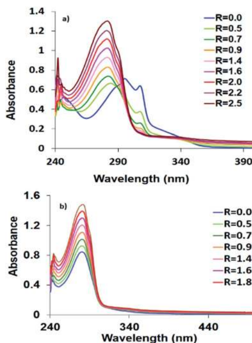
Fig. 4 Absorption spectra of complexes 2 (up) and 3 (down) in Tris-buffer (20% DMSO) in absence ( R = 0.0 ) and presence ( R > 0.0 ) of increasing amounts of HEWL ( R = [HEWL]/[\text{complex}] and [\text{complex}] = 1 \times 10^{-5} M).
