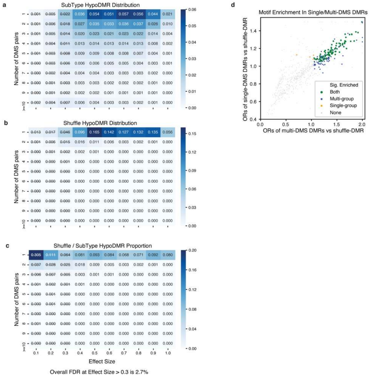
Extended Data Fig. 6 | Controlling the FDR of CG-DMRs. a, b. The proportion of subtype ( a ) or shuffled DMRs ( b ) in each block of specific effect size and number of DMSs. c. The empirical FDR of each block, calculated by (no. of shuffle-DMRs/no. of subtype-DMRs) in each block. DMRs with effect size <0.3 were excluded in further analyses. d. The odds ratio of transcription factor motif enrichment in single-DMS DMRs (sDMRs) and multi-DMS DMRs
