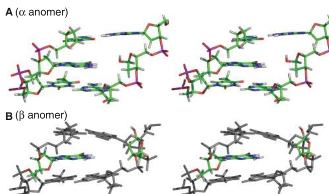
Figure 4. A stereo view of the conformation of the abasic site region in the averaged structure of Ab/G. (A) \alpha anomer. (B) \beta anomer. In B, only the abasic site and the unpaired bases are colored for clarity.
