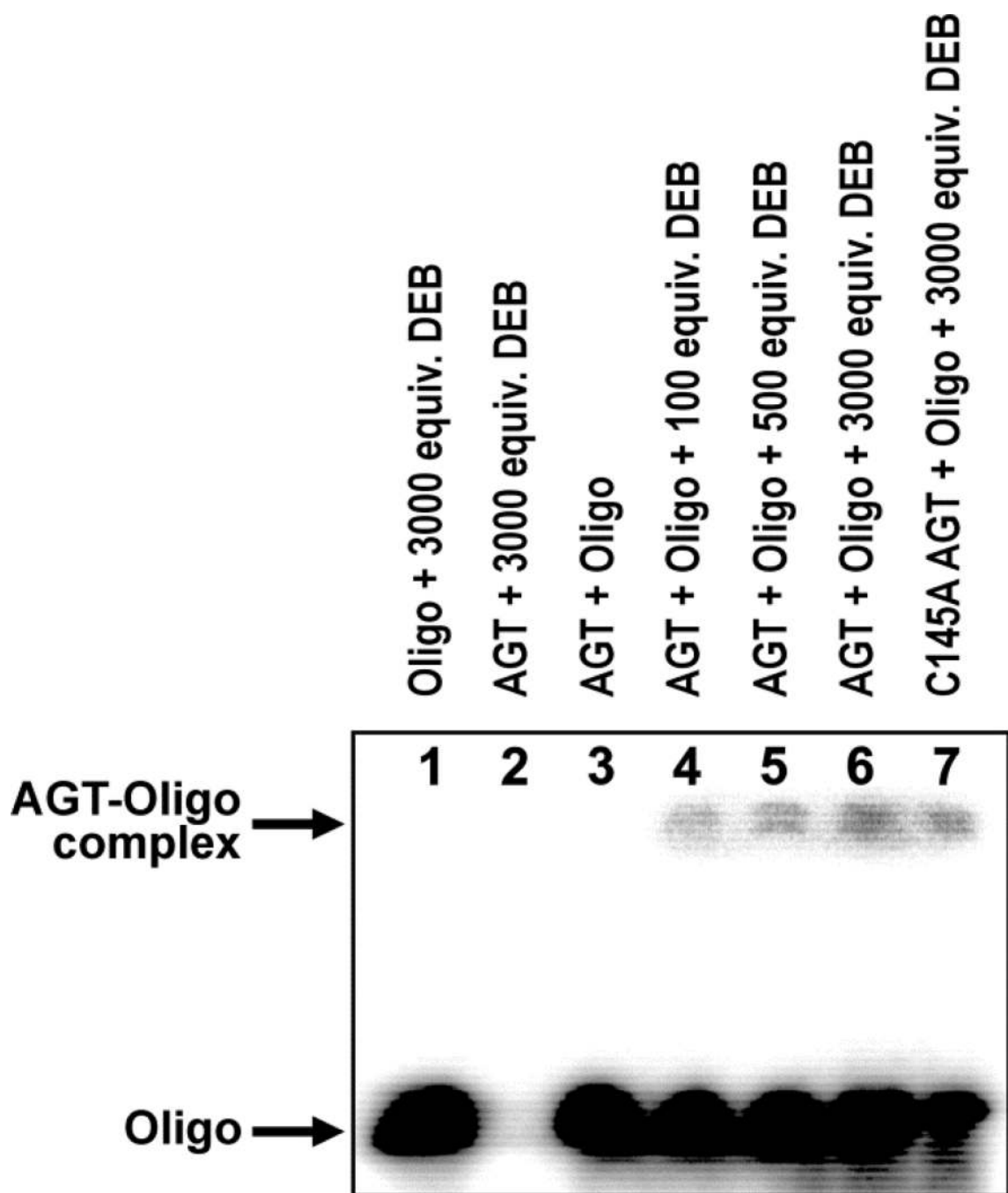
Figure 4. SDS-PAGE analysis of ^{32}\text{P} -endlabeled DNA duplexes (5'-GGA GCT GGT GGC GTA GGC-3', (+) strand) following incubation with DEB and hAGT (lanes 4–6) or C145A hAGT (lane 7). 42 AGT-DNA cross-links are observed as slowly moving bands on the gel. Lanes 1–3 serve as negative controls.
