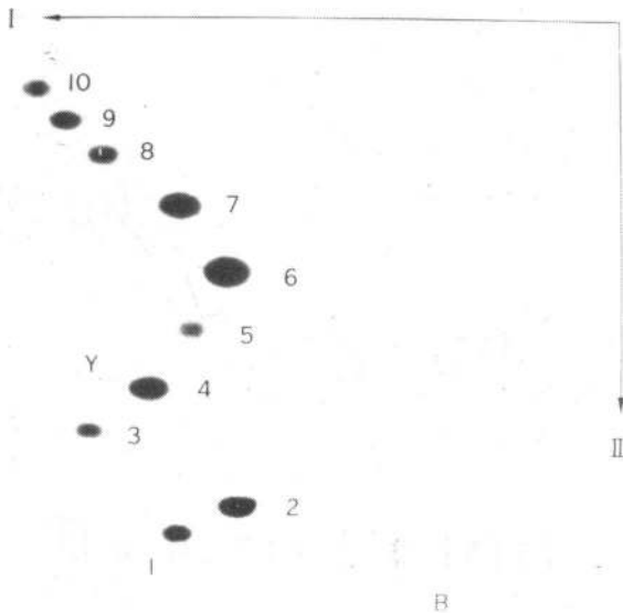
FIGURE 11 -- 2-D homochromatography (Homo-mix VI, 20 x 20 cm) fingerprint of the pancreatic DNase fragments of \lambda DNA labeled at the left-hand 3'-end with one d\text{-}^{32}\text{P} .
