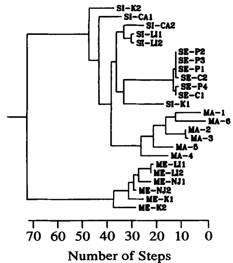
FIGURE 5.—A maximum parsimony tree. Branch lengths represent the number of steps required to construct the tree.
