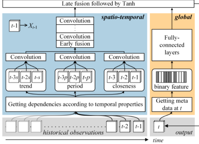
Figure 3: DeepST Architecture.
