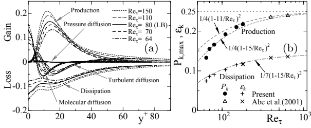
Figure 7: Budget of turbulent kinetic energy k normalized by \nu/u_\tau^4 ; (b) variation of the peak of production term P_{k,\max} and the dissipation rate \varepsilon_k at the same height.
