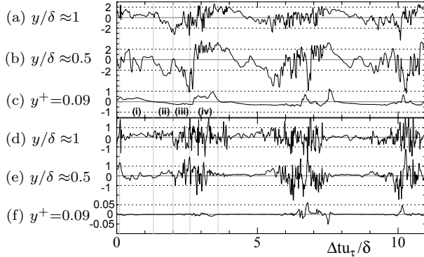
Figure 12: Typical time trace of u - and v -fluctuations at Re_\tau=80(\text{LB}) . The measurement points are at various wall-normal locations at the same position in the (x, z) -plane. (a)-(c), the streamwise fluctuation u^+ ; (d)-(f), the wall-normal fluctuation v^+ .
