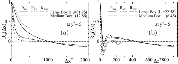
Figure 8: Two-point correlation coefficients R_{ii} of the velocity fluctuation component at Re_\tau = 80 ; (a) streamwise, (b) spanwise.
