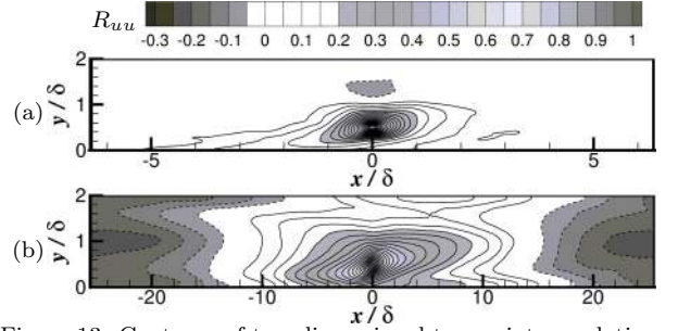
Figure 13: Contours of two-dimensional two-point correlation coefficient R_{uu} in the (x, y) -plane; the reference point is at the mid-height y_{\text{ref}} = 0.5\delta . The direction of the mean flow is from left to right. (a) Re_\tau = 180 ; (b) Re_\tau = 80 (LB). —, positive correlation; - - -, negative correlation; the line of R_{uu} = 0 is not shown here. Contour interval \Delta R_{uu}: 0.05 .
