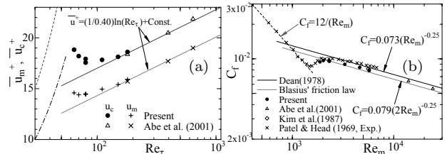
Figure 2: Reynolds number versus (a) centerline velocity u_c^+ and bulk mean velocity u_m^+ , (b) friction coefficient C_f . In (a), dotted lines (---, - · -) show the laminar flow relations of u_c = Re_\tau/2 and u_m = Re_\tau/3 , respectively.
