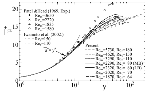
Figure 1: Mean velocity profile in viscous wall units
