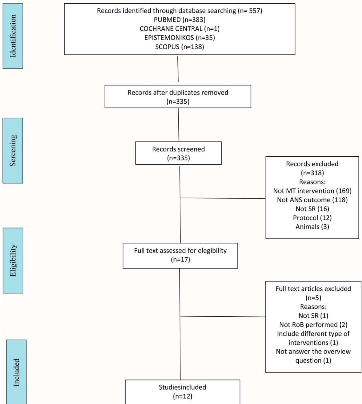
Fig 1. PRISMA flowchart.
