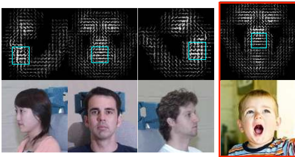
Figure 9: We show three rigid mixtures from a RMP model on the [left], along with their corresponding training images. RMPs share spatially-localized regions (or “parts”) between mixtures. Each rigid mixture is a superposition of overlapping parts. A single part is drawn in blue. On the [right], we show a mixture component which is implicitly synthesized by a DPM for a novel test image on-the-fly. In Fig. 10, we show that both sharing of parameters between mixture components and implicit generation of mixture components corresponding to unseen part configurations contribute to the strong performance of a DPM.
