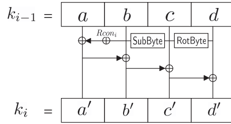
Fig. 2. Key Scheduling Algorithm of AES-128.
