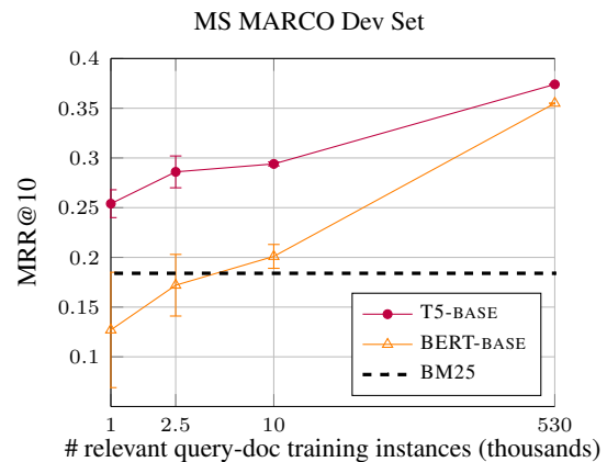
Figure 1: Comparisons between T5-base and BERT-base trained with different numbers of training instances (note the log scale in the x -axis). Results report means and 95% confidence intervals over five trials.
