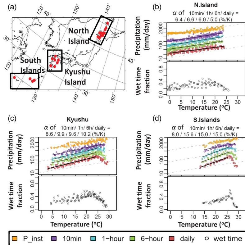
Figure 3. (a) Locations of three regions analyzed. Red circles in the map indicate the stations included for the analysis. (b, c, and d) The behaviors of P_{99\_10m} , P_{99\_1h} , P_{99\_6h} , P_{99\_d} , P_{inst} , and WTF are shown. The units of precipitations are converted to mm/day, and P_{inst} is multiplied by 10 for visibility. The values of \alpha for P_{99\_10m} , P_{99\_1h} , P_{99\_6h} , and P_{99\_d} estimated by exponential fitting are shown above each graph (Figures 3b–3d).
