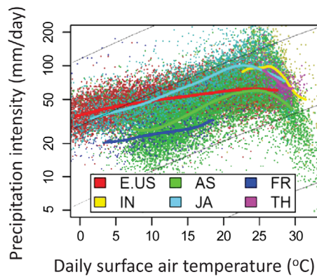
Figure 1. Behavior of P_{99,d} in six countries (Eastern United States (E.US), Australia (AS), France (FR), India (IN), Japan (JA), Thailand (TH)). “E.US” is the part of the United States extending from 22°N to 50°N and 65°W to 85°W. Each plot shows P_{99,d} for each T_a bin at each station. Thick lines denote the LOWESS smoothed lines for the six countries. CC scaling is illustrated by thin black lines for reference.
