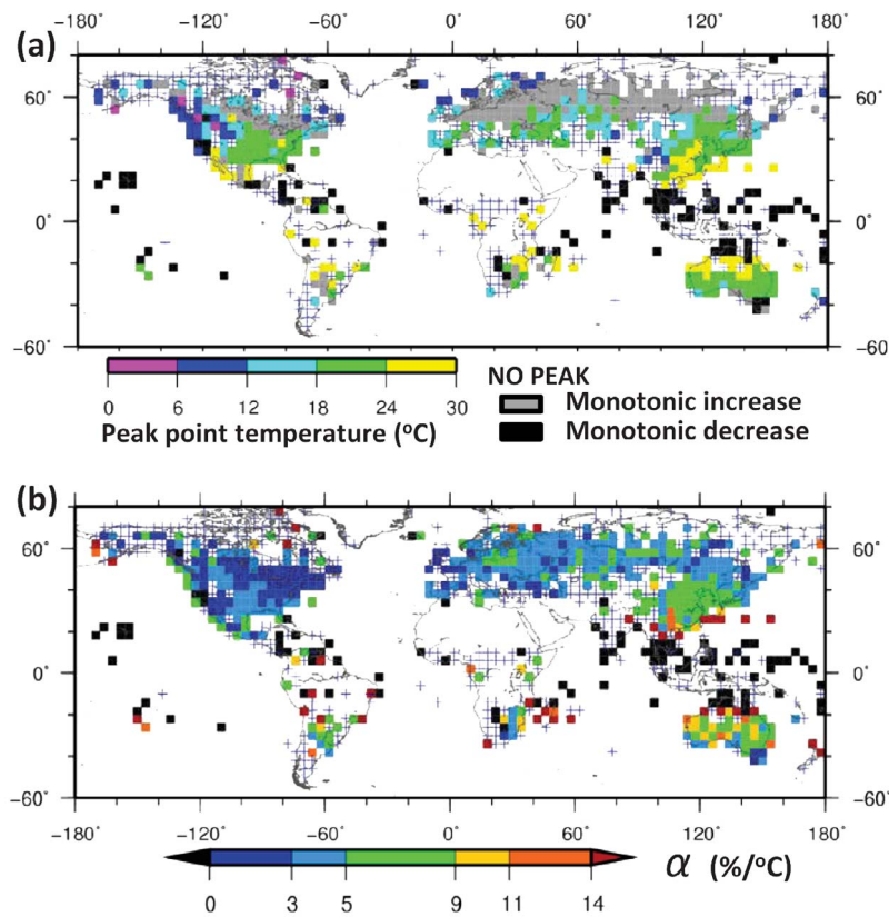
Figure 2. Global distribution of (a) peak-point temperatures and (b) \alpha for P_{99\_d} . The colored grid boxes have \alpha with 5% significance level. Grid boxes with no significance are indicated by crosses. White color indicates grids with no data suitable for the analysis.
