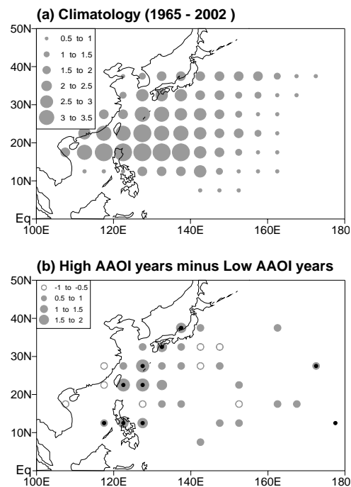
Fig. 2. Climatological distribution of tropical cyclone passage number (a) and difference between high AAO periods and low AAO periods in each 5^{\circ}\times 5^{\circ} longitude-latitude grid area (b). See Table 1 for detail information of high and low AAO periods. Mark \bullet indicates that the differences are significant at the 95% confidence level.
