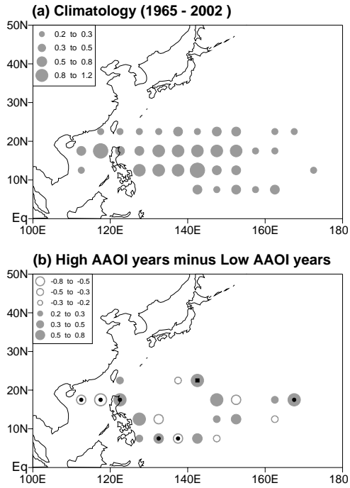
Fig. 3. Same as in Fig. 2 except for tropical cyclone genesis.
