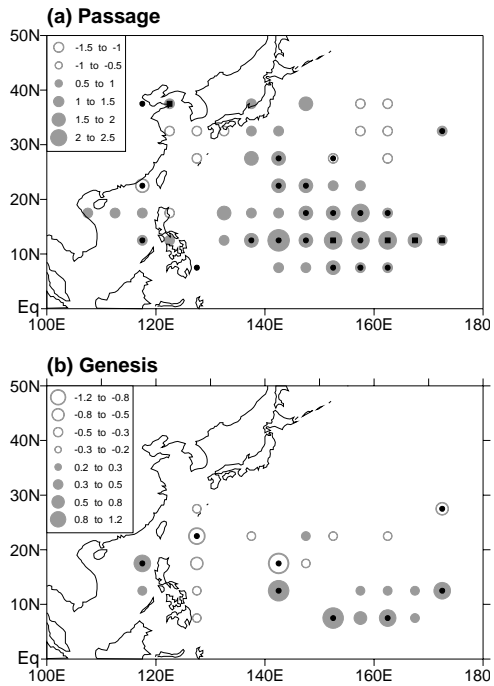
Fig. 4. Same as in Fig. 2 except for El Niño and La Niña years.
