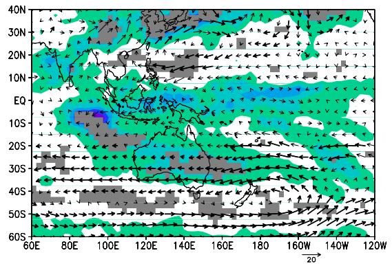
Fig. 5. Composite of moisture flux between high AAO years and low AAO years at 850 hPa. Decreased OLR is represented by shading.
