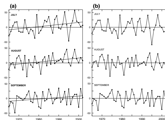
Fig. 1. Time series of leading EOF of monthly sea level pressure over the Southern Hemisphere (a) and detrended time series by subtracting the trend (b) for the period 1965-2002. The trends of the time series are shown in (a). The units are arbitrary.
