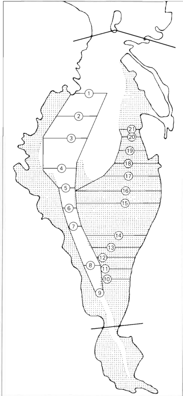
Fig. 2. Geometric approximation of the channel and eastern shoals of South Bay for calculating dispersive flux of chlorophyll (Equation 2). Chlorophyll was measured at all nodes (circles), where channel nodes (1 to 9) correspond to Stations 23 to 31 and shoal nodes (10 to 21) correspond to Stations 118 to 126 and 156 to 168
