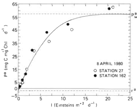
Fig. 3. Representative fit of Equation 5 to measured daily carbon assimilation rate at 7 light intensities. Equation 5 was fit here to pooled data from one sample collected in the channel and one sample from the eastern shoals
