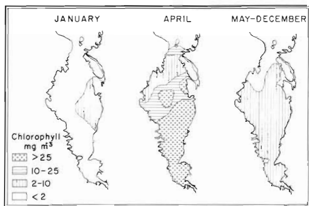
Fig. 4. Surface contours of chlorophyll a during winter, during spring bloom, and following spring bloom of 1980
