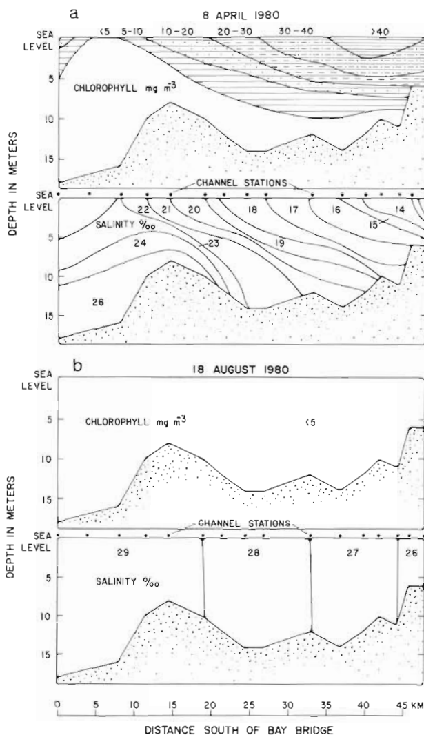
Fig. 5. Vertical contours of chlorophyll a and salinity along the South Bay channel: (a) during the brief spring period of salinity stratification; (b) during the remainder of the year
