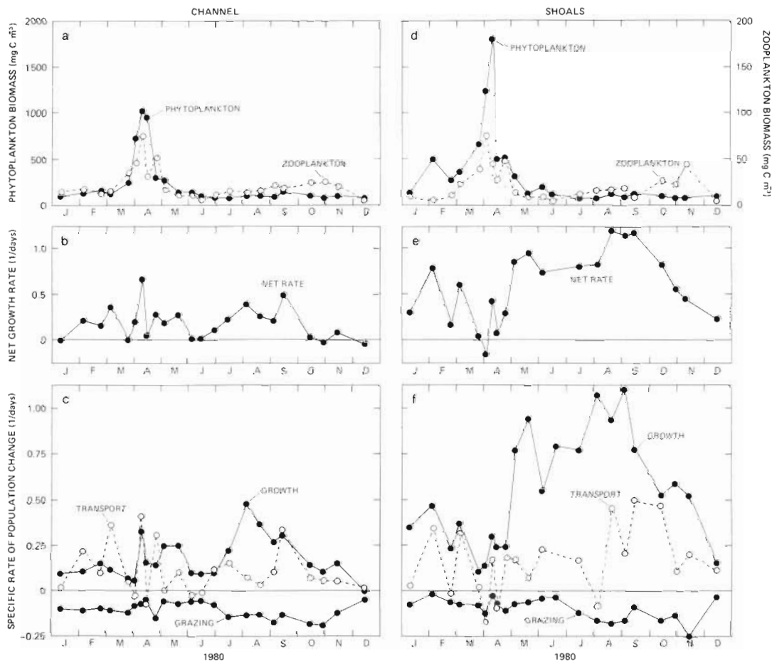
Fig. 6. Mean phytoplankton biomass (assuming a C:CL ratio of 49) and zooplankton biomass in the channel and eastern shoals of South Bay during 1980; phytoplankton biomass is the mean of surface values measured at Stations 23 to 31 (a) or 118 to 126 and 156 to 170 (d); zooplankton biomass is the mean of all samples collected at Stations 24, 27, 30 (a) or 118, 126, 156, 162, 168 (d). Net rate of phytoplankton population growth in the channel (b) and shoals (e). Calculated specific growth rate, transport rate, and zooplankton grazing rate in the channel (c) and shoals (f)
