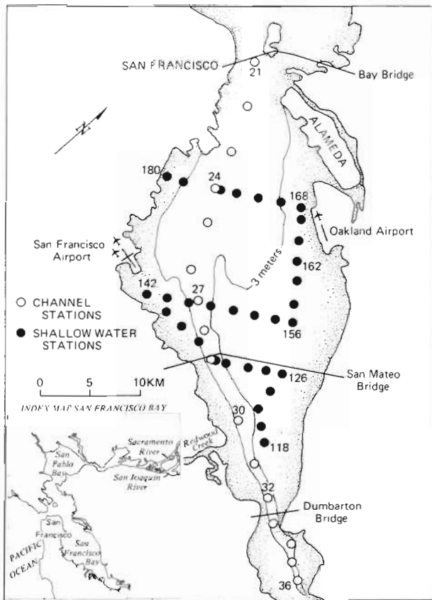
Fig. 1. Map of South San Francisco Bay showing locations of sampling sites in the channel (Stations 21 to 36) and across the shoals (Stations 118 to 180)
