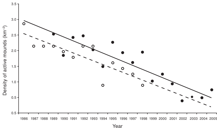
Fig. 1. The combined density of active Malleefowl mounds within six sites in SA (solid circles and solid line) between 1989–90 and 2005–06, and the density at Yalgogrin in NSW during the period 1986–87 to 1998–99 (open circles and broken line). Years on the x -axis refer to the beginning of the breeding season. The six sites in SA are Ferries-McDonald, Bakara, Cooltong, and Pooginook Conservation Parks, and Cowell and Shorts Heritage Agreements. Data for SA are taken from Gillam (2006); data for Yalgogrin from Priddel and Wheeler (2003).
