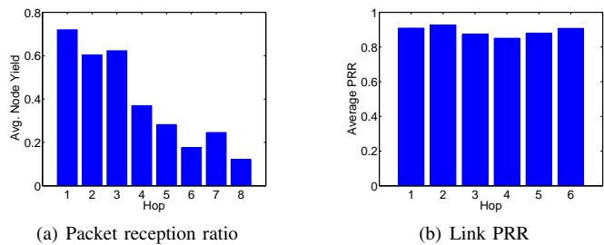
Fig. 4: System performance for different categories of nodes.
