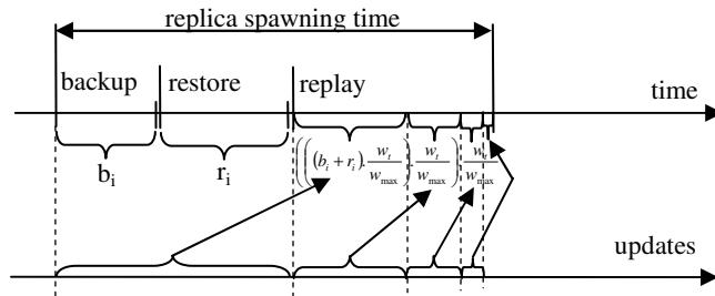
Figure 4. Decomposition of the replica spawning time with a new snapshot.
