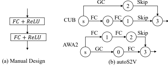
Figure 4. (a) The hand-designed architecture. (b) The learned task-specific architectures from autoS2V for CUB and AWA2, respectively. GC is the graph convolution.
