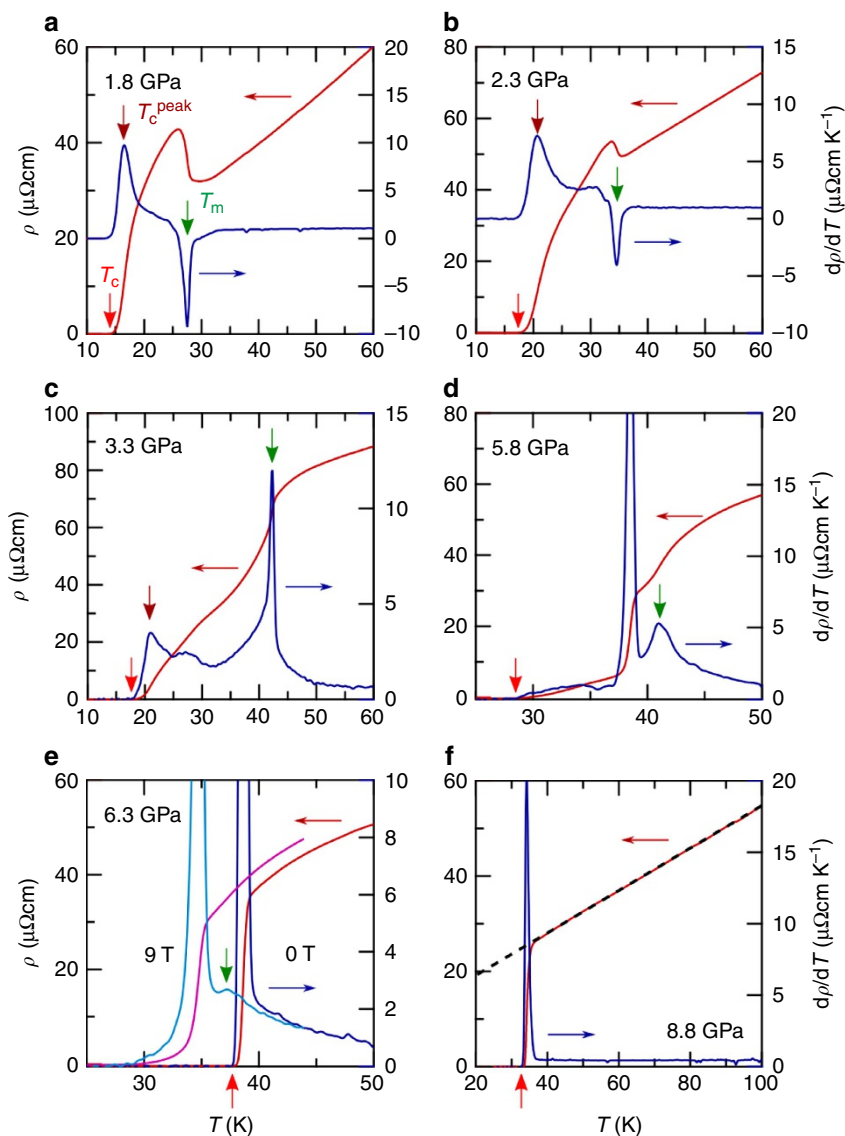
Figure 3 | Determination of magnetic and superconducting transition temperatures from the resistivity curves under high pressure. (a–f) Temperature dependence of resistivity \rho(T) (left axis) and temperature derivative of resistivity d\rho/dT(T) (right axis) at low temperatures. The temperature at the maximum slope of superconducting transition is defined as T_c^{\text{peak}} and the zero resistivity temperature as T_c . The magnetic transition temperature T_m is determined by the dip or peak in d\rho/dT(T) . At 6.3 GPa, the data at 9 T is also shown where T_m anomaly appears when the superconducting transition is suppressed to a lower temperature (e). At 8.8 GPa, the normal-state resistivity can be fitted to a T -linear dependence (dashed line in (f)).
