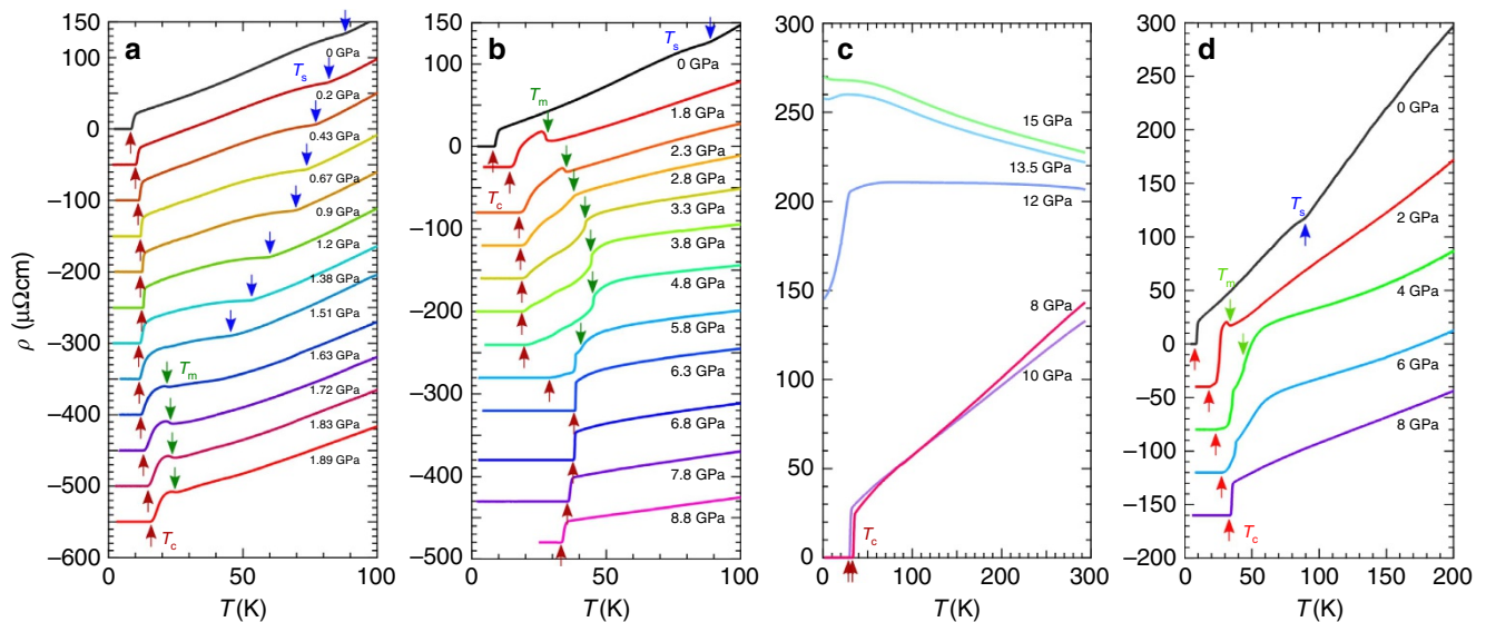
Figure 2 | Temperature dependence of resistivity in FeSe single crystals under high pressure. (a) \rho(T) curves below 100 K at different pressures up to \sim 1.9 GPa measured in the self-clamped PCC. (b) Data up to \sim 8.8 GPa measured in the self-clamped CAC. (c) Data up to \sim 15 GPa measured in the smaller self-clamped CAC. (d) \rho(T) curves below 200 K up to 8 GPa measured in the constant-loading CAC. Except for (c) the data are vertically shifted for clarity. The resistive anomalies at transition temperatures T_s , T_m , and T_c are indicated by the arrows.
