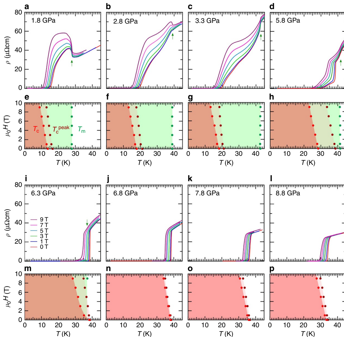
Figure 4 | Effects of magnetic fields on the magnetic and superconducting transitions under high pressure. (a-d, i-l) \rho(T) curves at different magnetic fields applied parallel to the c axis. The magnetic transition temperature T_m is field independent and marked by the green arrow (a-d). At 6.3 GPa, the T_m anomaly is only visible at high fields (i). (e-h, m-p) H - T phase diagrams. The zero resistivity is attained below T_c and the T_c^{\text{peak}} line (determined by the peak in d\rho/dT(T) ) is a lower bound of upper critical field H_{c2} . The sharp superconducting transitions under magnetic fields for P > 6.3 GPa indicate narrowed regimes of the vortex liquid state.
