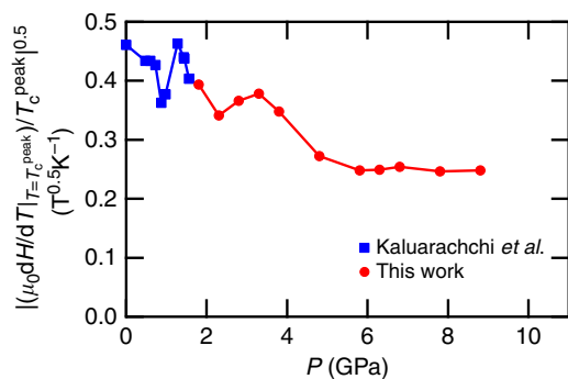
Figure 6 | Mass analysis from H - T curves under high pressure. The pressure dependence of the square root of the initial slope of the T_c^{\text{peak}} line divided by T_c^{\text{peak}} , which corresponds to the effective mass in a simple picture. For comparison, the low-pressure data from ref. 26 are also indicated (blue squares).
