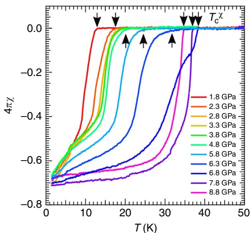
Figure 5 | Temperature dependence of ac susceptibility \chi under high pressure. The data are taken by using the clamp-type CAC. The onset temperatures T_c^\chi of diamagnetic signals are marked by arrows.
