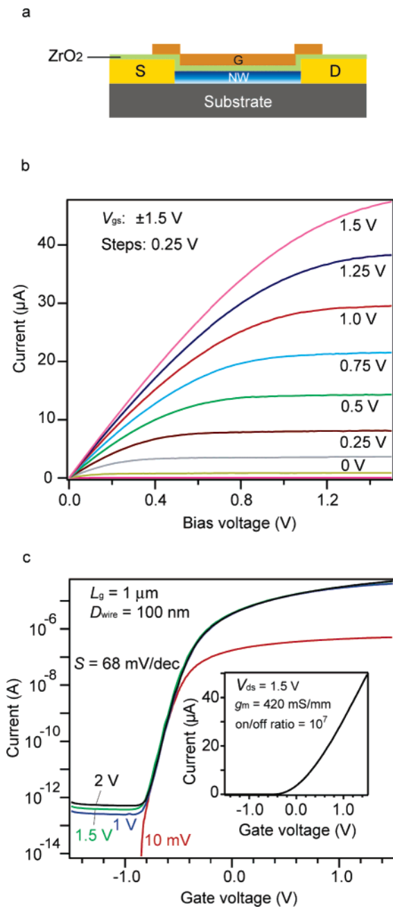
Figure 4. (a) Schematics of top-gate nanowire FET with \text{ZrO}_2 insulator layer. (b) I_{ds} - V_{ds} data of a 100-nm-diameter GaN/AlN/ \text{Al}_{0.25}\text{Ga}_{0.75}\text{N} nanowire with L_g = 1 \mu\text{m} at various V_{gs} values (from +1.5 V to -1.5 V, steps are 0.25 V). (c) Logarithmic scale I_{ds} - V_{gs} curves recorded at different V_{ds} = 2 \text{ V}, 1.5 \text{ V}, 1 \text{ V}, and 10 \text{ mV} , on the same GaN/AlN/ \text{Al}_{0.25}\text{Ga}_{0.75}\text{N} nanowire. Inset: linear scale I_{ds} - V_{gs} data recorded at V_{ds} = 1.5 \text{ V} .
