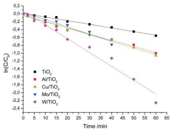
Fig. 8 Kinetic curves of RhB destruction over undoped and doped TiO 2 under visible light irradiation.
