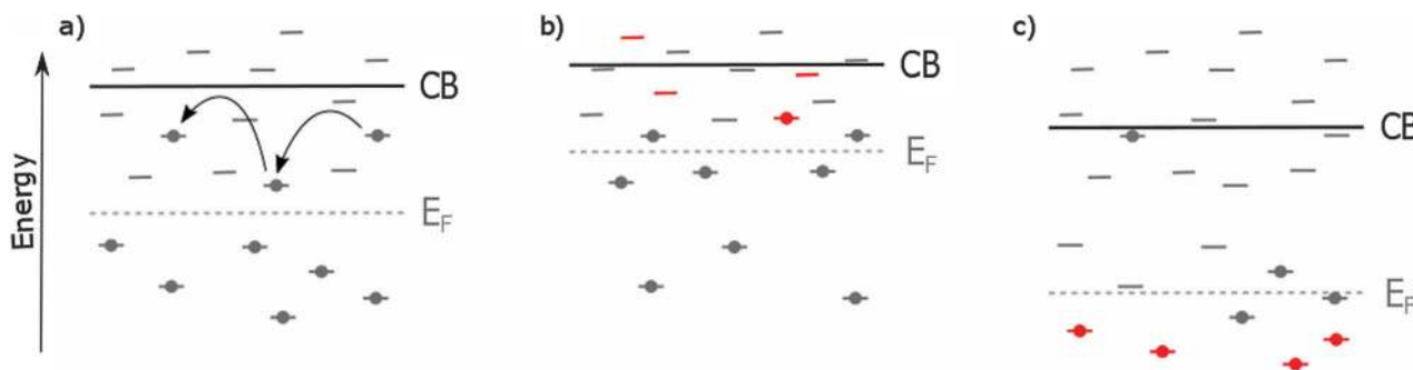
Fig. 3 The effect of \text{TiO}_2 doping on the CB and E_{\text{F}} . The doping induced states are shown in red. (a) In pristine \text{TiO}_2 , electrons are transported by 'hopping' from shallow trap to shallow trap until they reach the electrode. The shallow trap density will thus influence electron transport rate and J_{\text{SC}} . Deep traps can permanently trap electrons and act as recombination sites, affecting V_{\text{OC}} . Another important factor determining V_{\text{OC}} is E_{\text{F}} , as V_{\text{OC}} is defined as the difference between E_{\text{F}} of \text{TiO}_2 and the HTM. (b) Doping can decrease the deep trap density, resulting in an upward shift of E_{\text{F}} and thus an increase of V_{\text{OC}} . The elimination of deep traps retards recombination and boosts the V_{\text{OC}} even further. Because the CB is shifted towards the LUMO of the absorber, the driving force for electron injection is lowered, in combination with a decreased trap density and the related electron transport, lowering J_{\text{SC}} . (c) When doping contributes to the formation of deep traps, the conduction band and E_{\text{F}} are shifted downwards. In combination with enhanced recombination through the deep trap states V_{\text{OC}} decreases. Because of the larger offset between the CB and the absorber LUMO, electron injection is improved and the higher trap density causes an increase in electron transport, resulting in an enhanced J_{\text{SC}} . Ideally, the dopant eliminates deep traps while introducing new states close to CB, enhancing both V_{\text{OC}} and J_{\text{SC}} through decreased recombination and increased electron transport.
