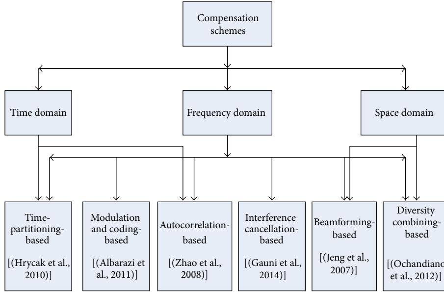
FIGURE 1: Taxonomy diagram for Doppler shift compensation schemes.
