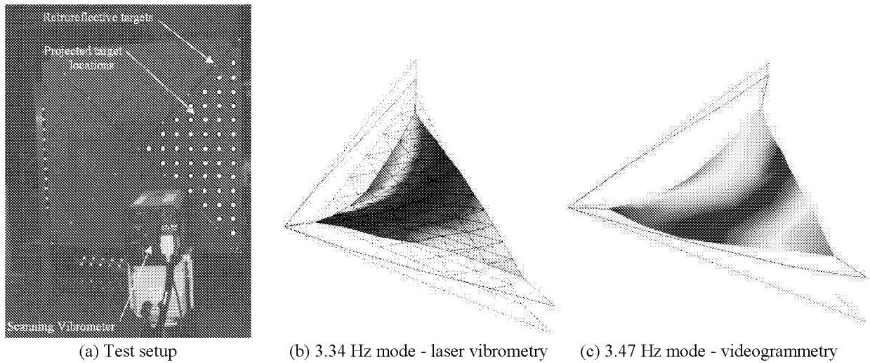
Figure 9. Videogrammetry of 2m matte-white solar sail quadrant with approximately 50 projected dots and comparison with corresponding laser vibrometry mode.
