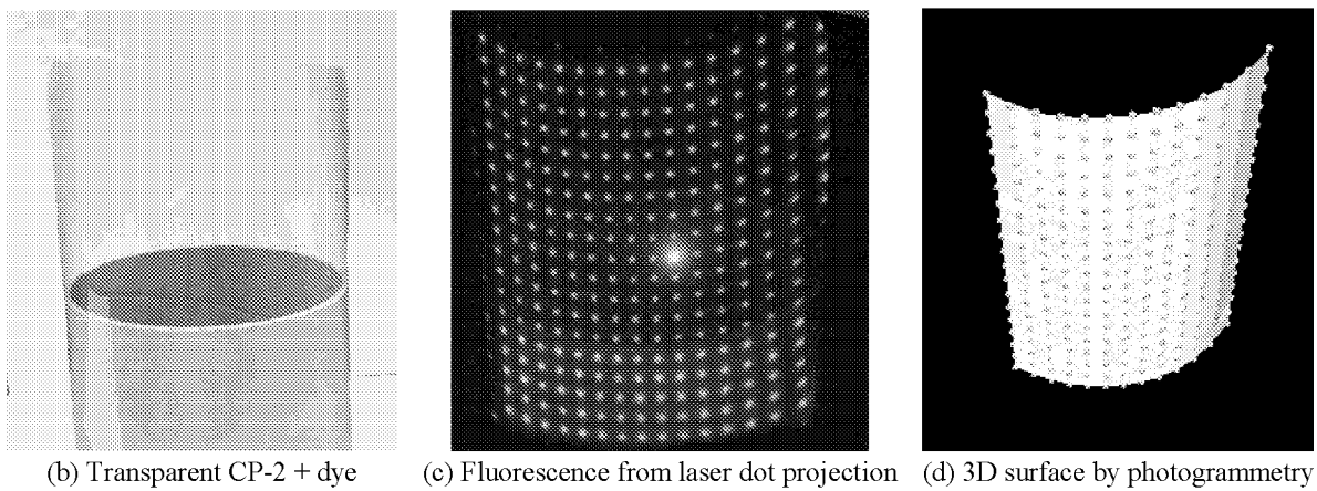
Figure 10. Laser-induced fluorescence for dot-projection photogrammetry of transparent membranes.
