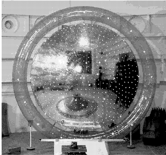
(a) 5m inflatable parabolic reflector
