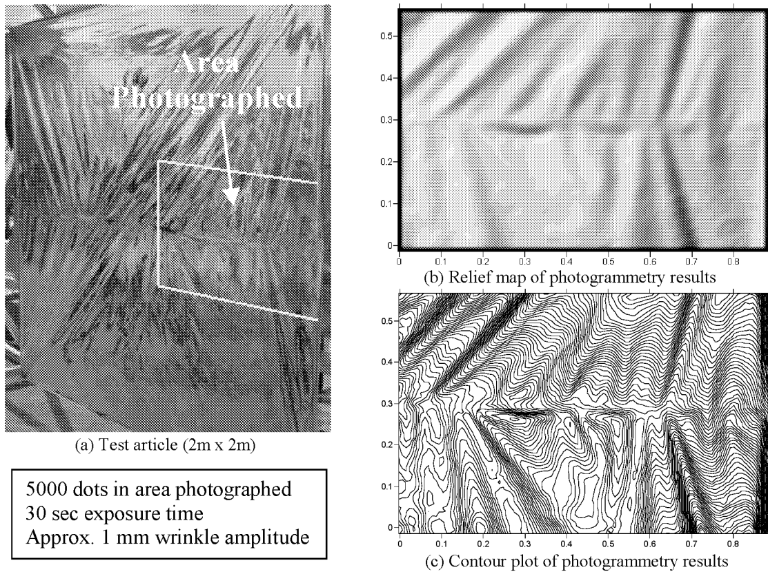
Figure 7. Photogrammetry of 2m aluminized Kapton solar sail using approximately 5000 projected dots.
