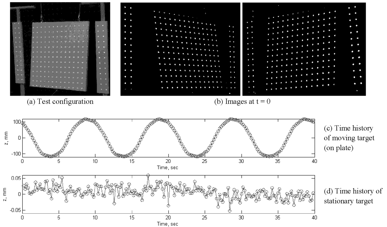
Figure 8. Videogrammetry of 0.6m oscillating white plate using approximately 200 projected dots.
