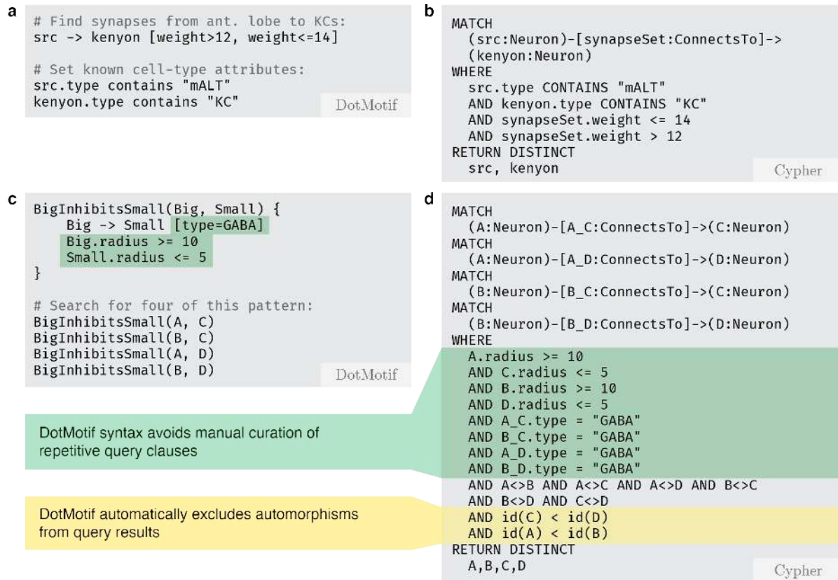
Figure 6: A comparison of DotMotif query syntax and the equivalent queries when transpiled to Cypher using the Neo4jExecutor. a. A simple query to find inputs to Kenyon cells ( KC ) from the medial antennal lobe tracts ( mALT ) in the Hemibrain dataset. Note that DotMotif comments are notated with the hash character. b. The equivalent query as panel a , when converted to the Cypher query language for use with neuPrint systems. Even in a small query such as this, DotMotif syntax tends to be more succinct and readable. c. A simple DotMotif query for a repeated pattern with node and edge constraints. The motif includes a macro called BigInhibitsSmall , which establishes a connection between two neurons with a type edge-attribute of “GABA”, and with radius nodes attribute constraints on both neuron participants. This macro is reused multiple times in the final motif construction in order to avoid repetitive code. DotMotif automatically infers that nodes A and B are isomorphic (i.e. interchangeable), and that C and D are isomorphic. d. DotMotif converts the query in panel c to the Cypher code in d . The equivalent Cypher query is substantially longer and harder to maintain or edit, even in the case of this quite simple motif. It also requires explicit notation to avoid reporting duplicate motif automorphisms.
