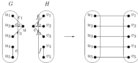
Fig. 6. 5-edge expansion.
