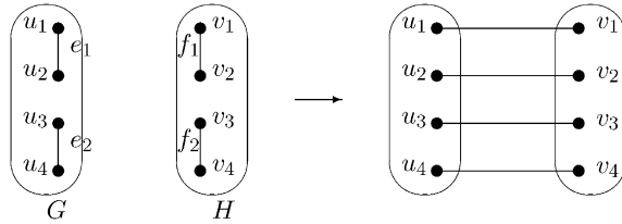
Fig. 5. 4-edge expansion.
