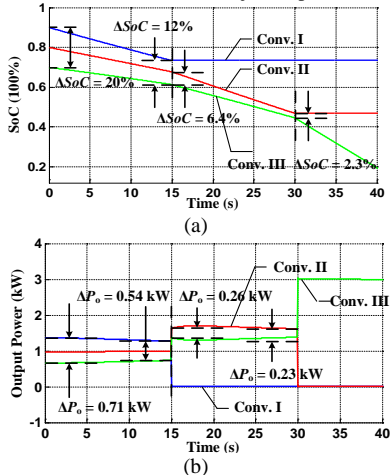
Fig. 15. Discharging process with dynamic disconnection of ESUs.
