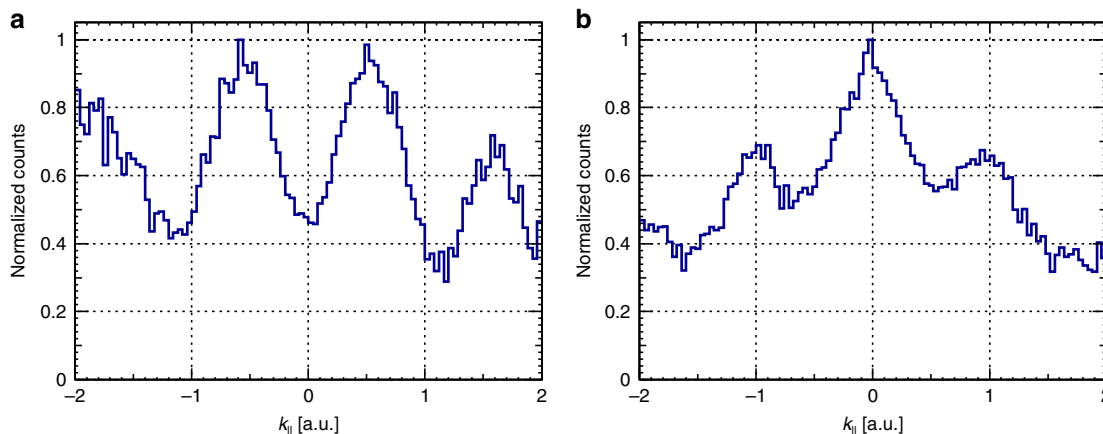
Fig. 3 Photoelectron momentum distributions of \text{Ne}_2 for linearly polarized light. Normalized photoelectron momentum distributions projected to the molecular axis for the direct (a) and indirect (b) dissociation pathways in case of linearly polarized light. The spectra were generated by selecting only the events, where the dimer axis lies within \pm 15^\circ to the polarization direction of the laser field. In addition, the ion momenta were limited to 4.5–16 a.u. and 39–45 a.u. for the direct and indirect dissociation, respectively. Original spectra were divided by the corresponding spectrum of the monomer in order to remove the ionization weighting. k_{\parallel} is the electron momentum component parallel to the dimer axis
