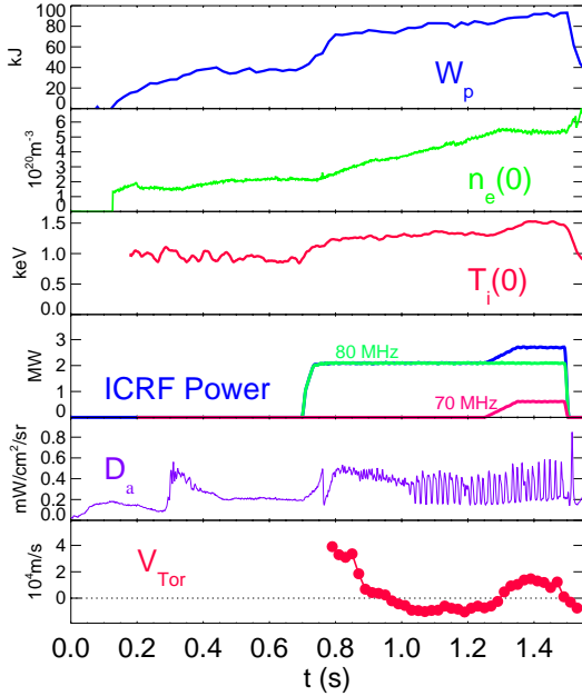
Fig. 1: Parameter time histories for a double barrier plasma. In the top panel is the plasma stored energy, and in the 2 nd and 3 rd panels are the central electron density and ion temperature, respectively. In the 4 th panel is the ICRF power at 80 MHz (green) and 70 MHz (red), with the total shown in blue. D_\alpha emission is shown in the 5 th frame and in the bottom panel is the central toroidal impurity rotation velocity.
