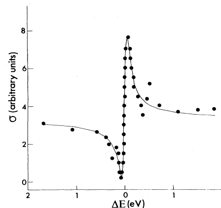
FIG. 4. The 1s^2 1S - 2s2p \ 1P resonance of \text{Li}^+ . The points represent a typical set of experimental data. The line shows the computer output for the calculated profile. For the particular set of data used the values of q and \Gamma were -1.31 and 0.074 eV, respectively (least-squares values). The triangular instrumental function had a full width at half-maximum of 0.08 eV.
