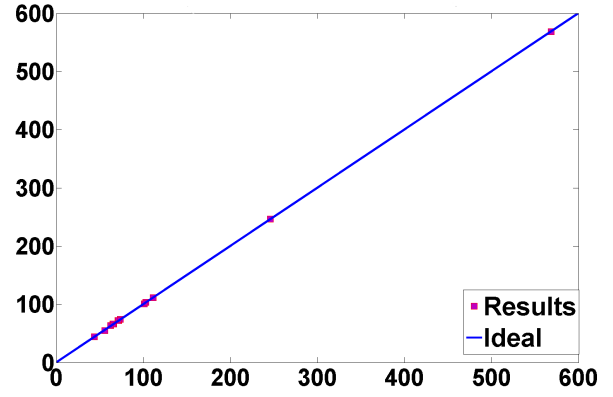
Figure 3: Real Inverse Epidemic Threshold ( \lambda_1 ) vs. our estimate for 14 different datasets . As we see, the estimates are almost ideal, in most cases differing in the second decimal digit. Similar results hold for other graphs as well.
