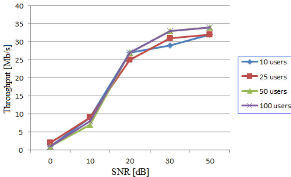
Figure 5.19 SNR versus Throughput for multiple users.
