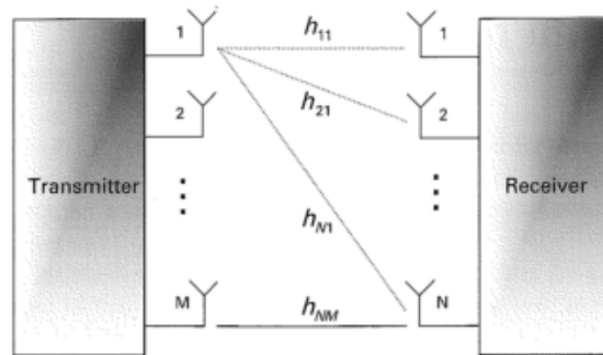
Figure 2.6 MIMO systems [10]
