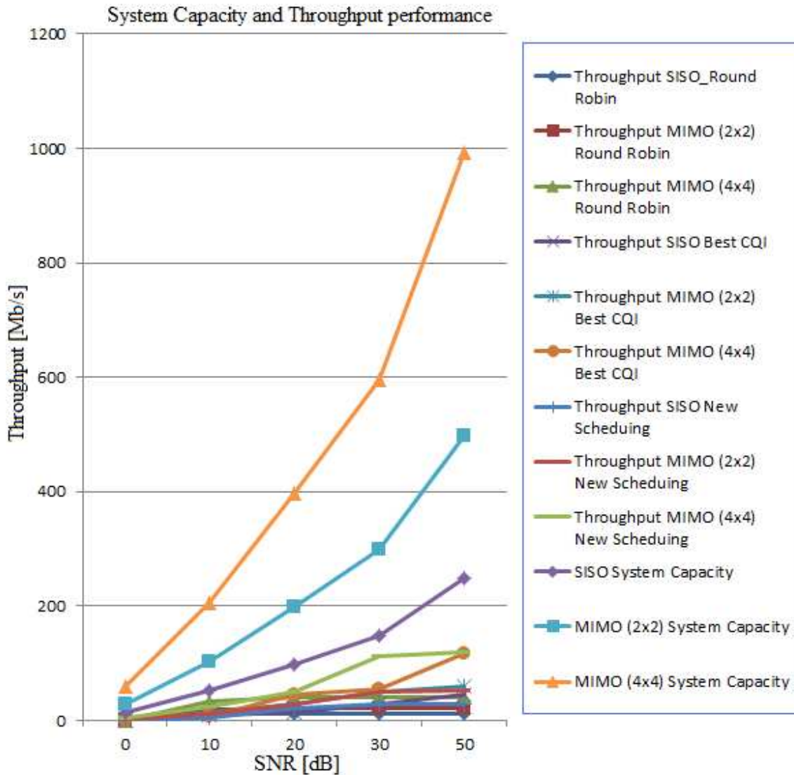
Figure 5.15 Channel capacity and throughput for a single user.
