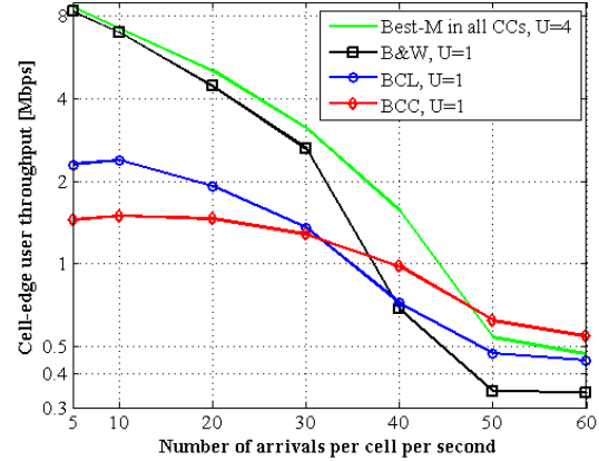
Fig. 6. Cell-edge user throughput with a smaller payload size of 1 Mbts.
