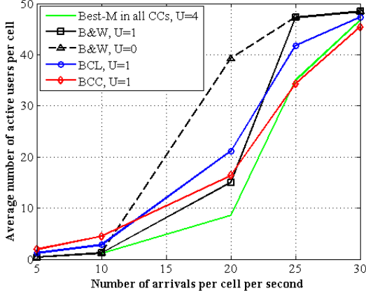
Fig. 3. Number of active users with various Poisson arrival rates. Payload size is 2 Mbts. For cross-CC CQI reduction, maximum one CC is reported using the best-M CQI compression scheme.
