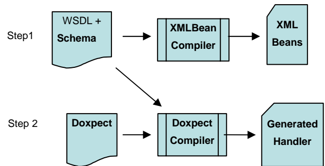
Figure 5: Doxpect Tool Process (From left to right, programming artifacts, tools, binary output).
