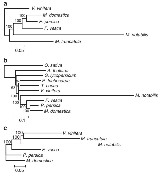
Figure 4 | Phylogenetic trees of M. notabilis and other plants. Different data sets were used to construct a phylogeny of the considered species. (a) A tree constructed using 136 single genes in the predicted M. notabilis gene data sets and their best-matched ones. (b) A tree constructed using 62 single genes predicted by Genewise in 10 plants. (c) A tree constructed using 318 best-matched collinear genes across 6 plant genomes. The scale of a unit is shown below each tree and the number on it shows how many amino acid substitutions per sites.
