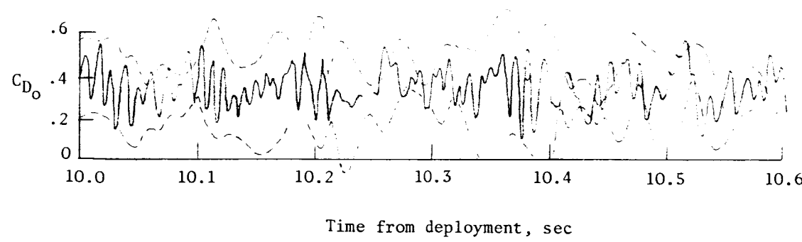
Figure 10.- Time histories of drag coefficients at M = 2.0 for 12.5-percent geometric porosity model behind cylindrical base extension for three different periods during a test.
