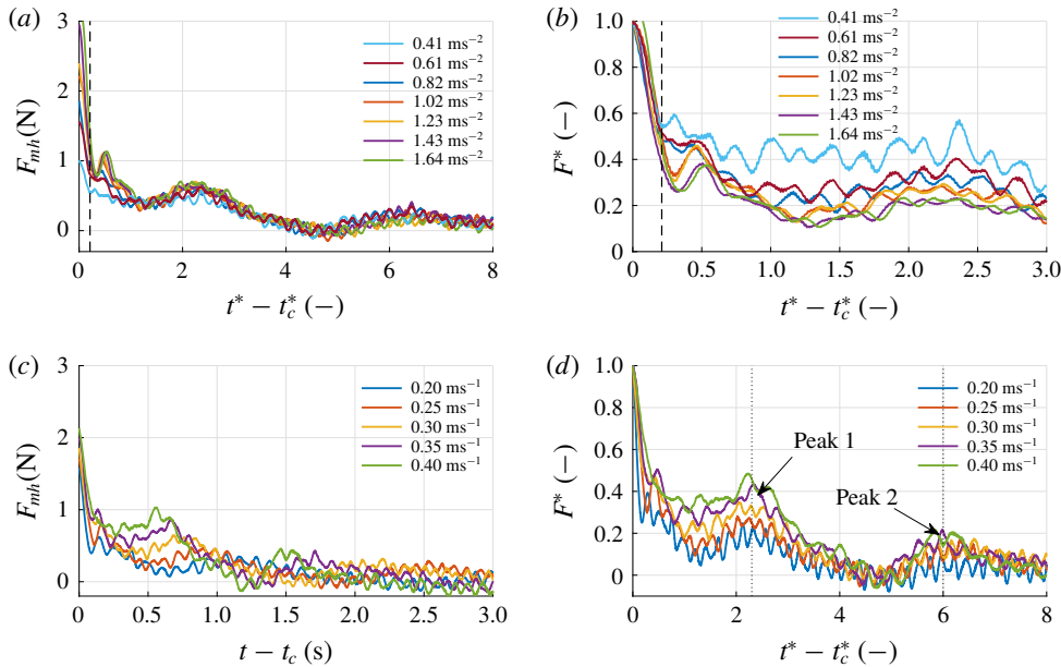
FIGURE 12. (Colour online) The residual force in dimensional form F_{mh} (a,c) and non-dimensional form F^* (b,d) as a function of the post-acceleration time t - t_c or formation time t^* - t_c^* for different accelerations towards a fixed plate velocity V = 0.30 \text{ m s}^{-1} (a,b) or towards different velocities at a fixed acceleration a = 0.82 \text{ m s}^{-2} (c,d) for plate depth h = 100 \text{ mm} . In (a,b) the dashed line indicates the dimensionless step response time t_{sr}^* . In (d) the dotted lines indicate the locations of peak 1 and peak 2 which for different velocities coalesce in non-dimensional time. (a) Residual force as function of post-acceleration formation time for h = 100 \text{ mm} , velocity V = 0.30 \text{ m s}^{-1} and varying accelerations. (b) Normalised residual force as function of post-acceleration formation time for h = 100 \text{ mm} , velocity V = 0.30 \text{ m s}^{-1} and varying accelerations. (c) Residual force as function of post-acceleration time for h = 100 \text{ mm} , acceleration a = 0.82 \text{ m s}^{-2} and varying velocities. (d) Normalised residual force as function of post-acceleration formation time for h = 100 \text{ mm} , acceleration a = 0.82 \text{ m s}^{-2} and varying velocities.
