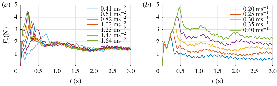
FIGURE 10. (Colour online) Drag force signals F_x(t) measured at plate depth h = 100 \text{ mm} . (a) F_x(t) for various accelerations towards a fixed plate velocity V = 0.30 \text{ m s}^{-1} . (b) F_x(t) for a fixed acceleration of a = 0.82 \text{ m s}^{-2} towards various plate velocities V .
