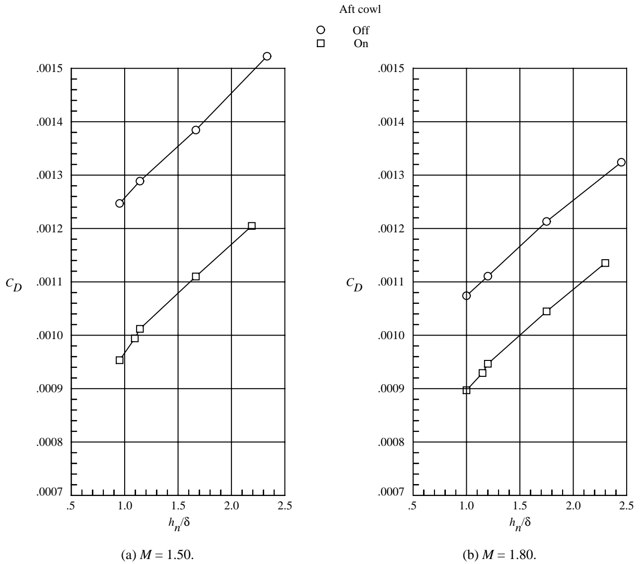
Figure 8. Effect of aft cowl on nacelle drag at \theta = 8.0^\circ .
