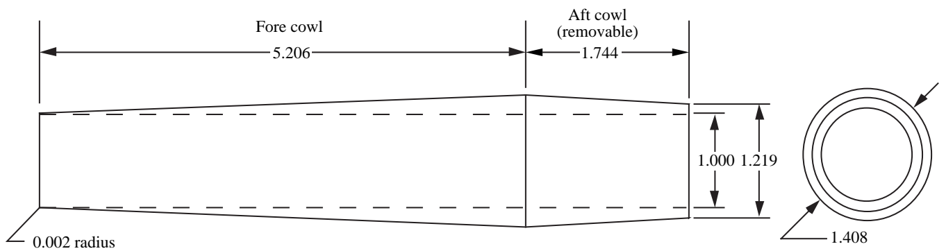
(c) Sketch of nacelle. All linear dimensions are given in inches.
