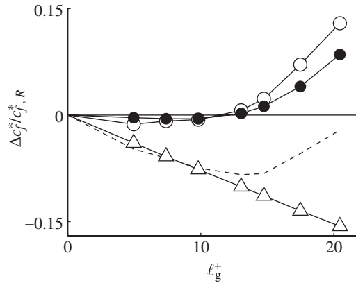
Figure 7. Break-up of the drag reduction curve, as defined in equation (4.1). Open triangles, slip term; open circles, full Reynolds stress term; filled circles, Reynolds stress term calculated only within the spectral region outlined in figure 6a; dashed line, full approximate drag reduction, \Delta c_f^*/c_f^* .
