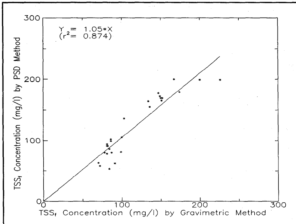
Figure 5. Comparison of TSS_f measured by gravimetric method to TSS_f measurement by PSD method
