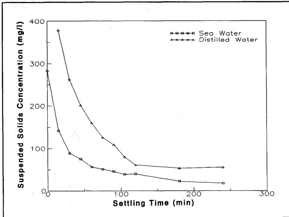
Figure 23. Settling behavior for TSS_1 concentrations of 0.5 g/l
