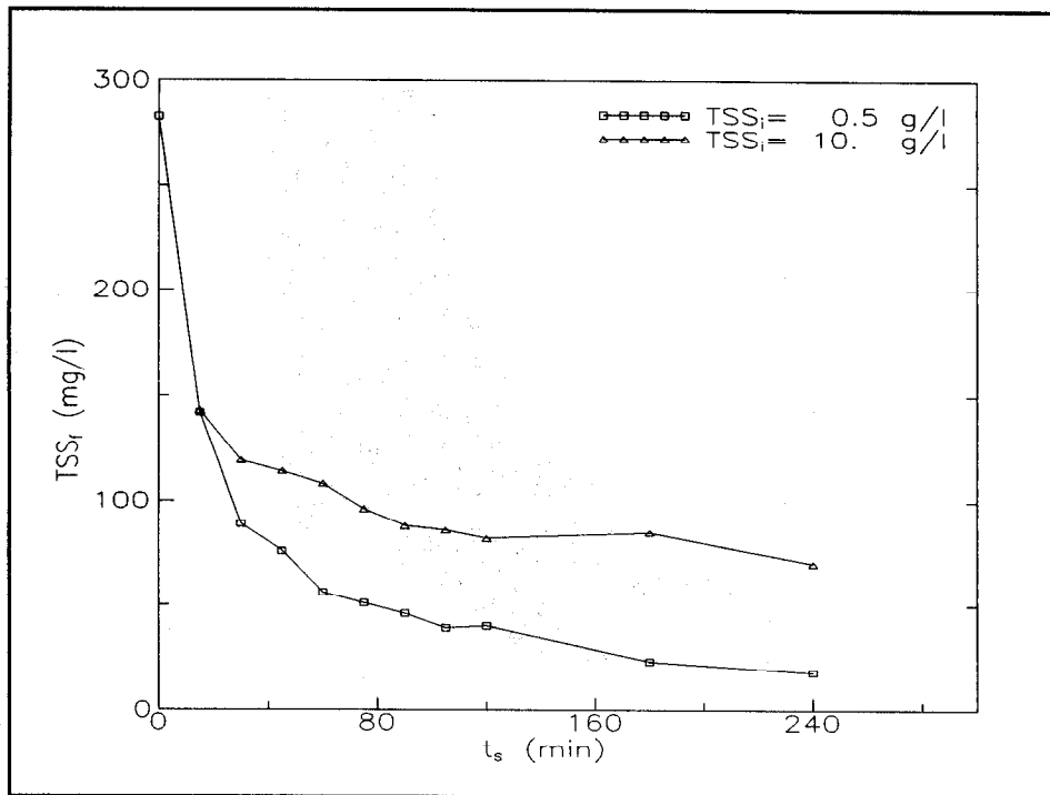
Figure 6. TSS_f as a function of time after a 1-hr aeration time
