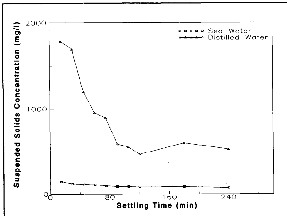
Figure 24. Settling behavior for TSS_1 concentrations of 10 g/l
