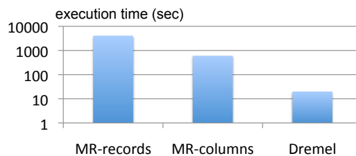
Figure 10: MR and Dremel execution on columnar vs. record-oriented storage (3000 nodes, 85 billion records)
