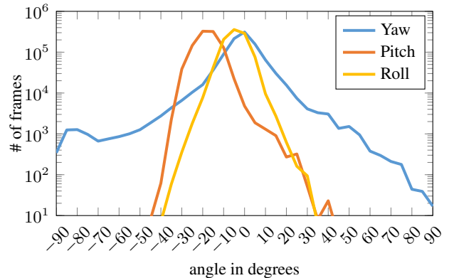
Figure 4: Histogram of DriveAHead frames for yaw, roll and pitch angle.
