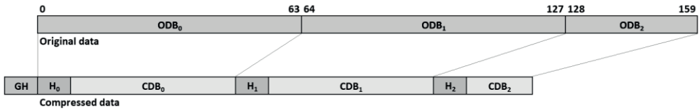
Figure 1. The original data consisting of 160b is divided into blocks with a length of 64b. Two blocks of a standard length 64b were created – named ODB 0 and ODB 1 . the last block named ODB 2 is shorter and has a length of 32b. Compressed data consists of three Compressed Data Blocks (CDB) labeled CDB 0 to CDB 2 each with its own header labeled H 0 to H 2 . There is a Global Head (GH) of the whole data structure in its introductory part.
