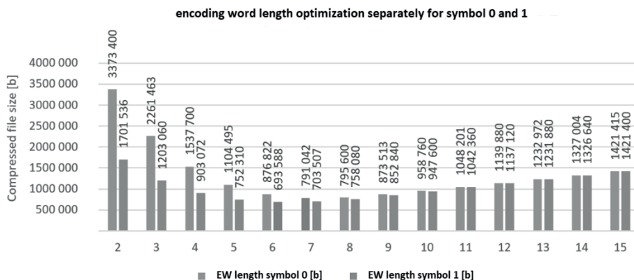
Figure 12. Optimization of EW length dissociated for symbol 0 and 1 allows to choose the optimal length of EW from the range of < 2; 15 > b , for symbol 0 and for symbol 1, separately. As it can be seen from the graph, for particular dataset the optimal length of EW for symbol 0 is 7b and for symbol 1 is 6b . In that case the data after compression represent the smallest file size ( 693\ 588\ b + 791\ 042\ b = 1\ 484\ 630\ b ).
