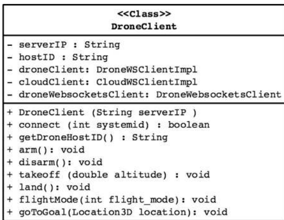
Fig. 8. DroneClient UML class diagram.
