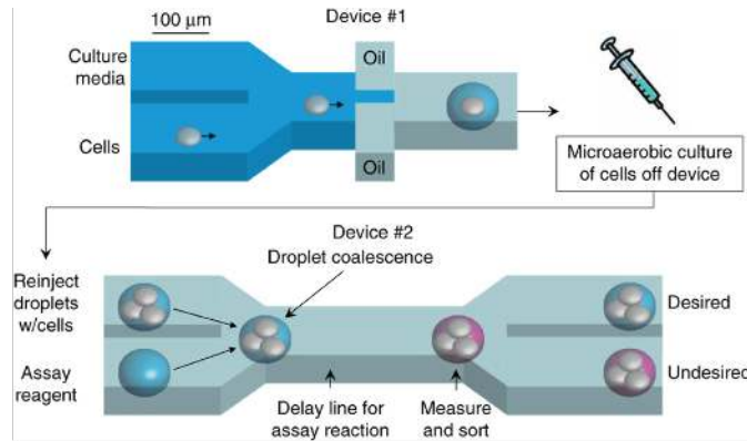
Figure 2. Droplet-based microfluidics and cell biology. Initially, droplets containing cells and culture media are generated and collected in a syringe that provides a micro-aerobic environment when capped. The syringe is placed in an incubator for cell culturing. Subsequently, the droplets from the syringe are reinjected into another microchannel structure, where they are merged with another set of droplets containing fluorescent enzymatic assay reagents. After a delay, the reaction begins in the merged droplets. The droplet fluorescence is measured using a laser/detector system. Consequently, the extracellular concentration of the metabolite of interest is quantified. This system can screen one to two clones per second. The figure is reproduced, with permission, from Wang et al. [34].
