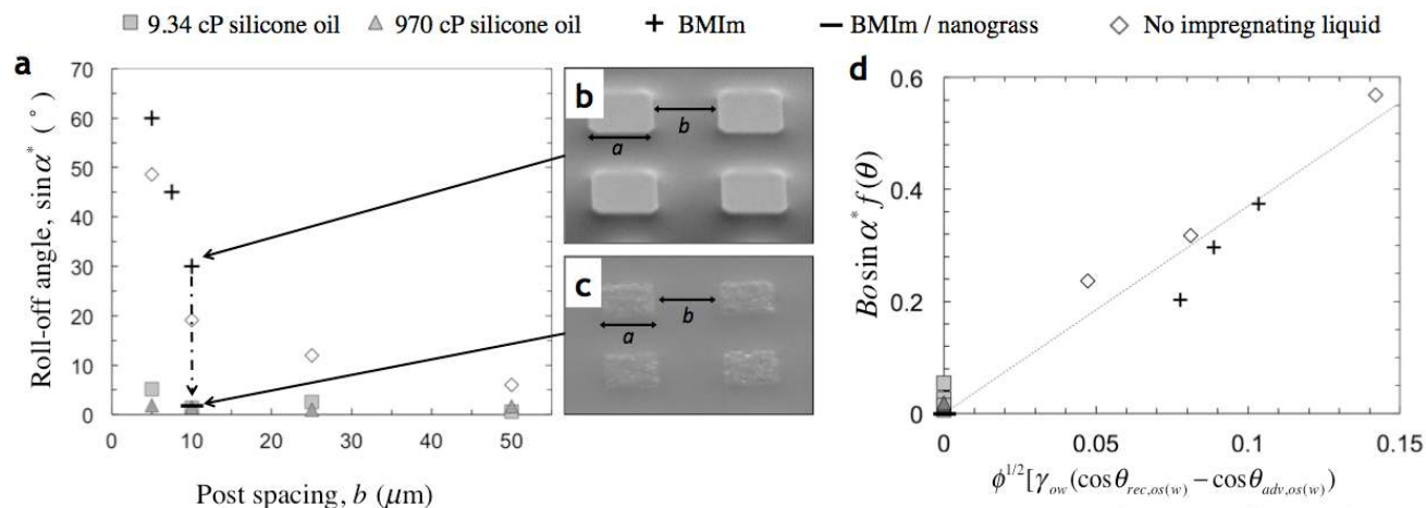
FIG. 3. (a) Measured roll-off angles for different encapsulating liquids as a function of post spacing b . Extremely low roll-off angles are seen in the case of silicone oil impregnated surfaces, consistent with the post tops being encapsulated both outside and underneath the droplet (state A3-W3 , \theta_{os(a)}, \theta_{os(w)} = 0 ). The high roll-off angles seen in the case of BMIm impregnated surfaces are consistent with the post tops being emergent outside and underneath the droplet (state A2-W2 , \theta_c > \theta_{os(a)}, \theta_{os(w)} > 0 ). (b) The top inset shows an SEM image of the BMIm impregnated texture and reveals that the post tops are dry. (c) When the posts are further roughened by adding nanograss, they are covered with BMIm (bottom inset) and consequently, the roll-off angle decreases. (d) Non-dimensional plot of scaled gravitational force (left side of Eq. (11)) at the instant of roll-off as a function of the relevant pinning force (right side of Eq. (11)) shows that the roll-off data is in general agreement with the scaling.
