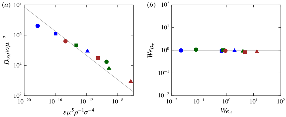
FIGURE 9. (Colour online) (a) Normalized maximum droplet size D_{95} as a function of the energy input \varepsilon . The grey solid line is the relation \rho\sigma D_{95}/\mu^2 = 0.725(\mu^5\varepsilon/\rho\sigma^4)^{-2/5} proposed by Hinze (1955). (b) Critical Weber number We_{D_{95}} based on the maximum droplet size D_{95} for all the cases considered.
