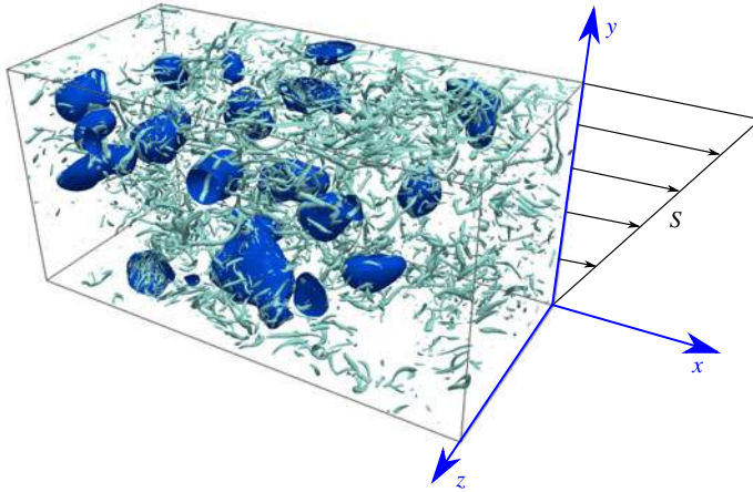
FIGURE 1. (Colour online) Sketch of the computational domain and of the Cartesian coordinate system. The visualization pertains to flow at Re_z \approx 15\,000 with 5% volume fraction of the dispersed phase at We_\lambda \approx 0.75 . The blue colour is used to depict the surfaces of the droplets.
